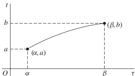
FIGURE 37 t = \phi(\tau)
