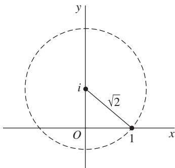
FIGURE 79 |z-i| < \sqrt{2}
