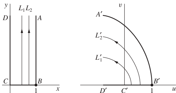
FIGURE 134 w = z^2.
