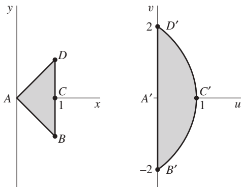
FIGURE 137 w = z^2 .
