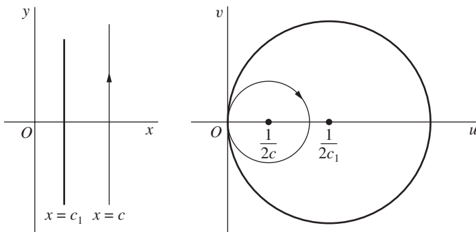
FIGURE 120 w = 1/z .
