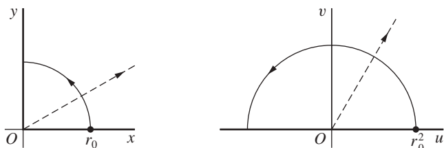
FIGURE 21 w = z^2 .
