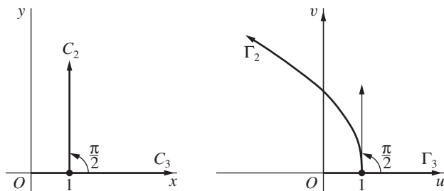
FIGURE 150 w = z^2 .
