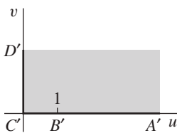
FIGURE 10 w = \sin z.
