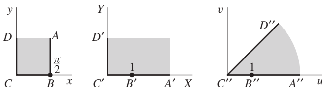
FIGURE 138 w = F_0(\sin z) .
