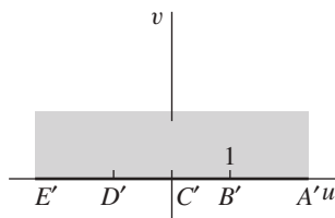
FIGURE 9 w = \sin z.
