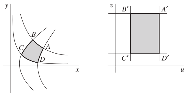
FIGURE 2 w = z^2 .
