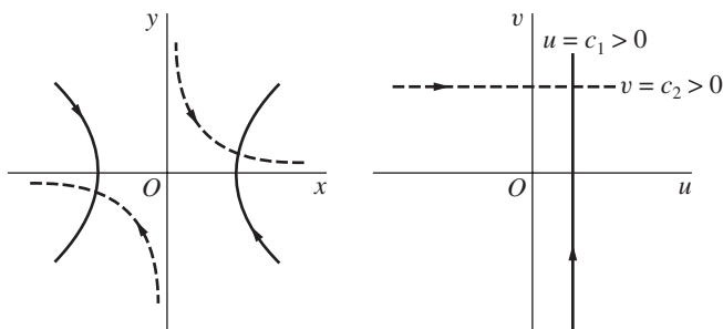
FIGURE 19 w = z^2 .
