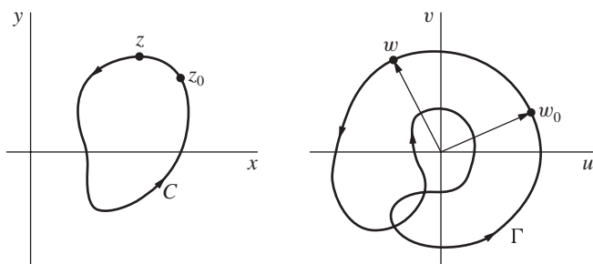
FIGURE 113
