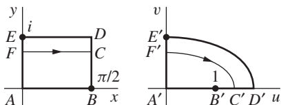
FIGURE 132 w = \sin z .
